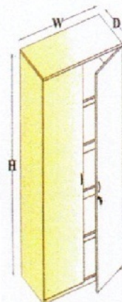
HIGH SWING DOOR W=900, 750, 600 D=450, 450, 500, 550, 600 H=1800, 1800, 2100
