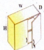
OVER HEAD STORAGE W=450, 750, 900, 1050, 1200 D=300, 350, 380, 400, 450 H=1500, 1800, 1800, 2100
